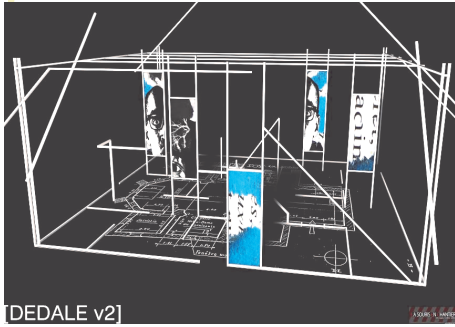
DEDALE v2]
